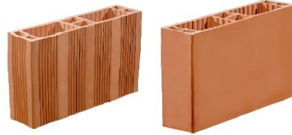
LADRILLO PERFORACION VERTICAL No. 3 - NO ESTRUCTURAL
